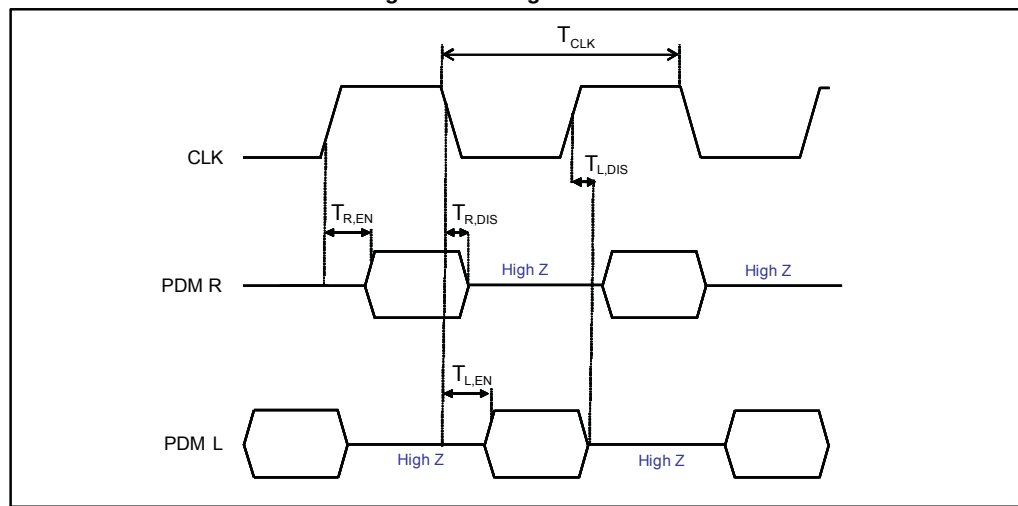
Figure 2: Timing waveforms
