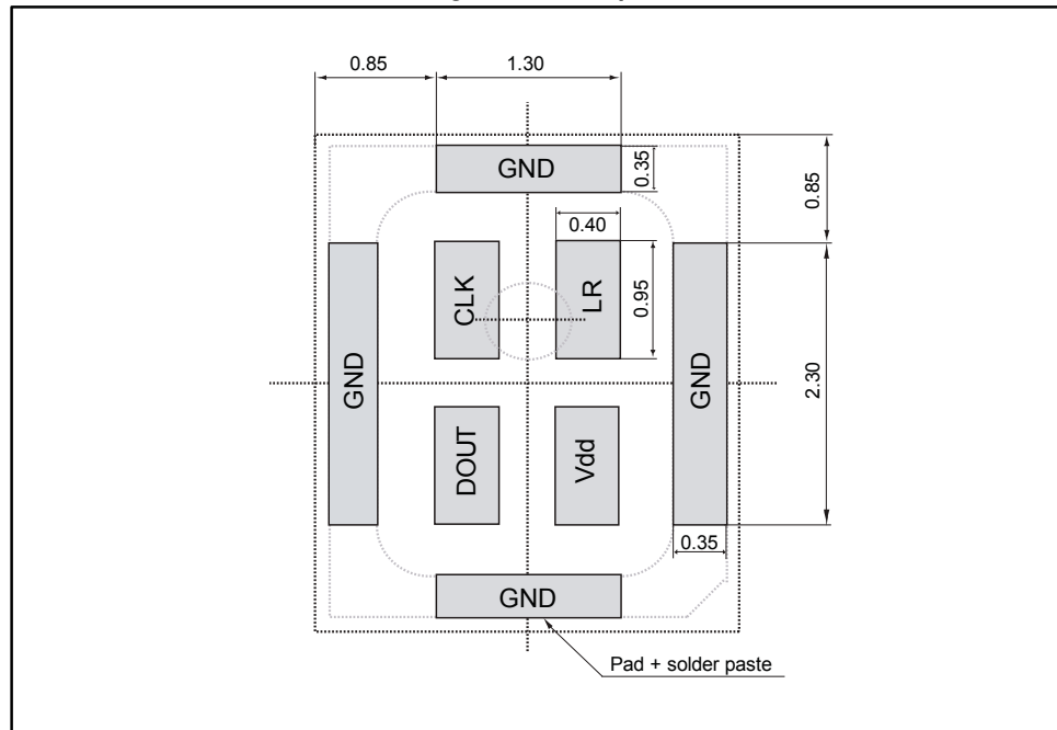
Figure 12: Land pattern
